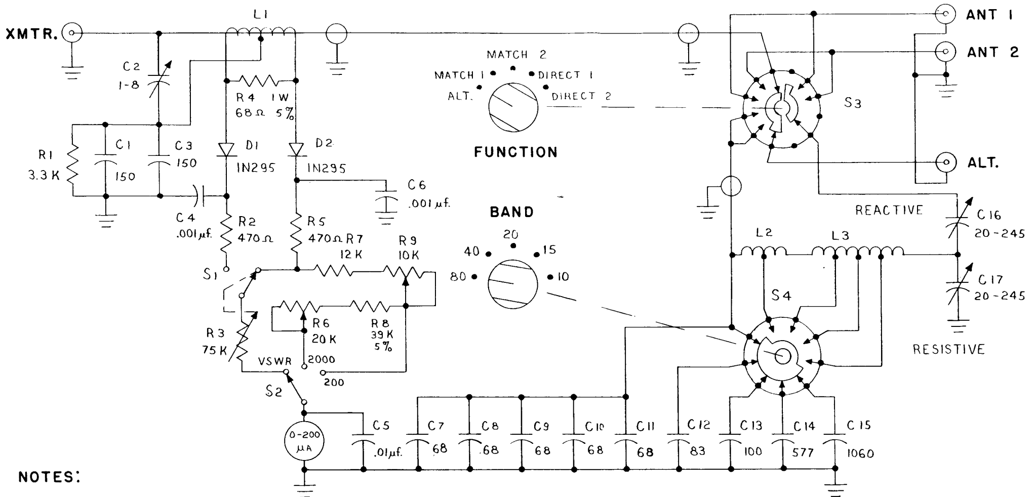
SCHEMATIC DIAGRAM MODEL MN-2000 MATCHING NETWORK
